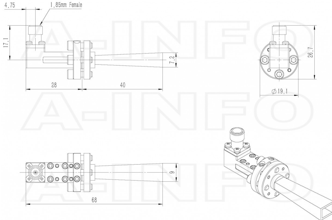
1.85mm-Female Output (P/N: LB-15-10-C-1.85F)
